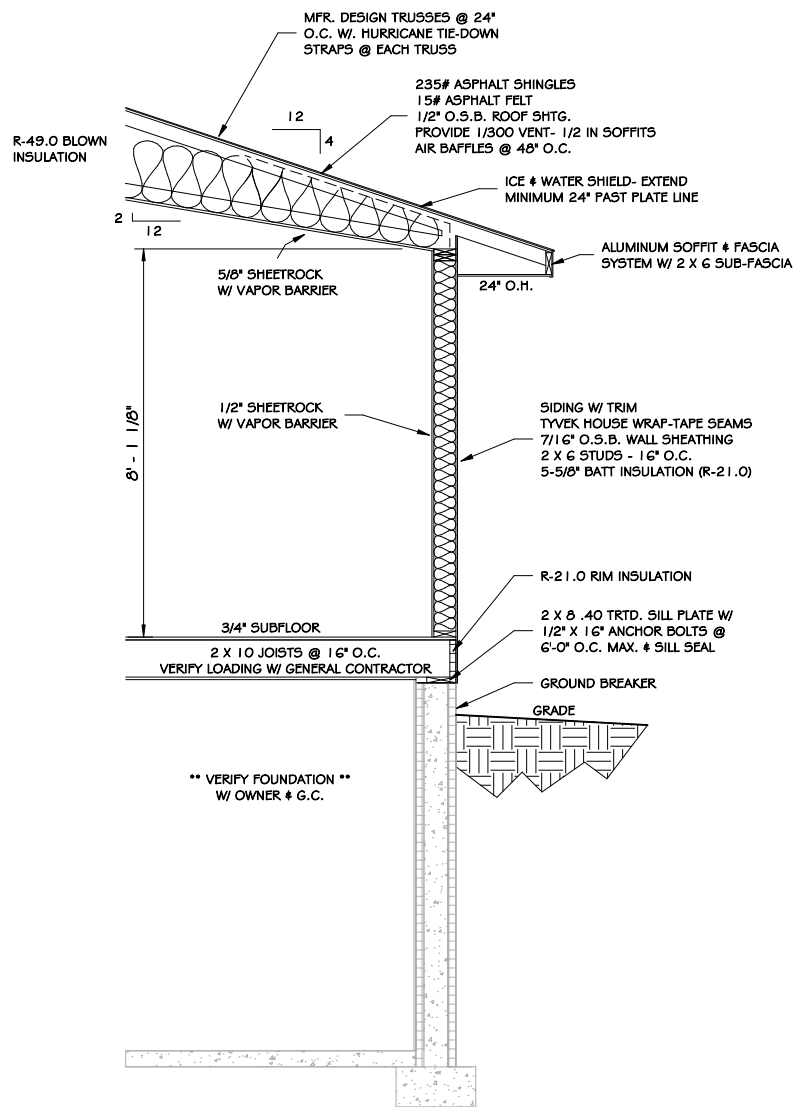
2 WALL SECTION 1/4" = 1'-0"
