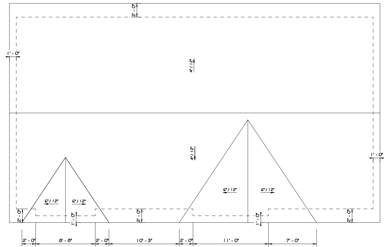
1 ROOF PLAN 1/8" = 1'-0"
