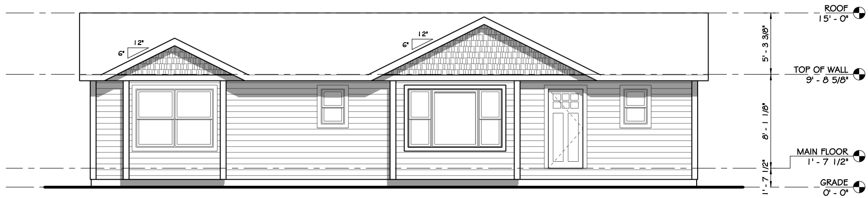
1 FRONT ELEVATION AI 1/8" = 1'-0"
