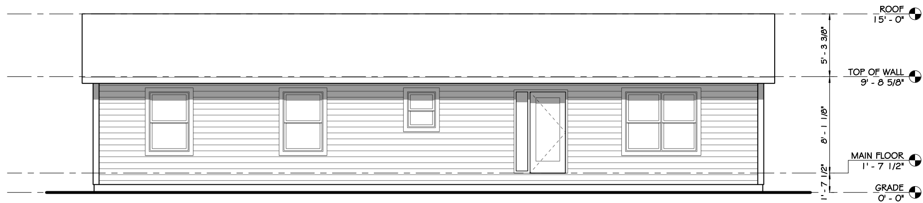
1 FRONT ELEVATION AI 1/8" = 1'-0"
